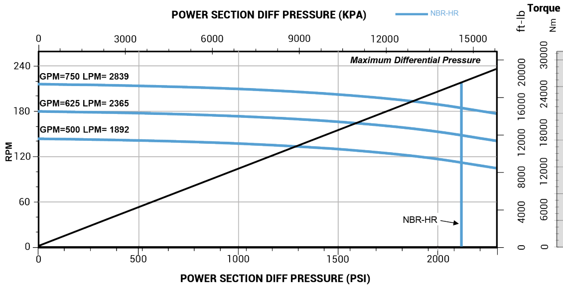
Titan 22 7" 7/8 9.4 Power Curve
